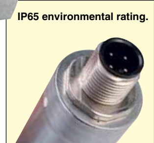
PX459, M12 connector.
